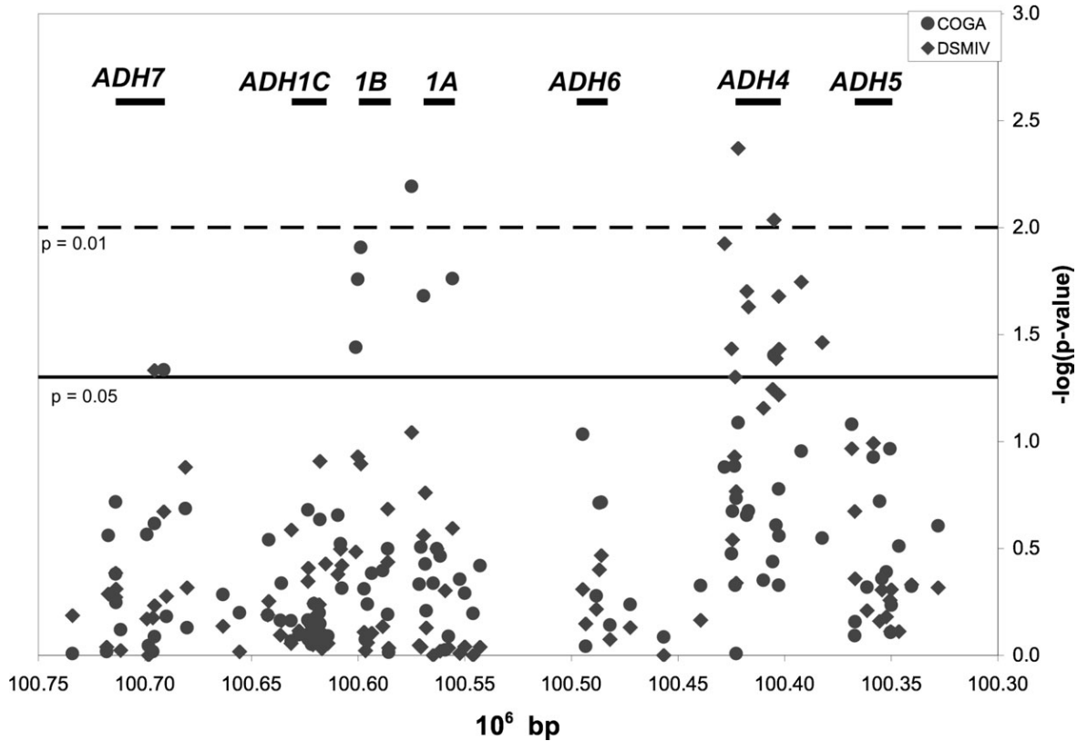
Figure 2. Association of SNPs across the ADH gene cluster with alcohol dependence. Results of the PDT_{sum} are plotted as -\log(P\text{-value}) . Diamonds represent results with DSM-IV definition of alcohol dependence and circles represent results using COGA criteria. Locations of the ADH genes are shown as lines across the top; genes are transcribed from left to right; abscissa runs from qter toward cen.
