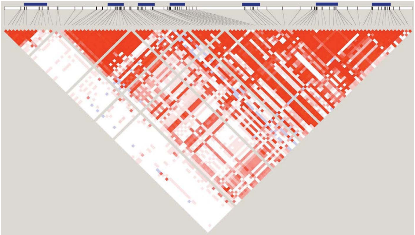
Figure 1. LD ( D' ) between the SNPs genotyped in the ADH cluster: Haploview. Blue lines at top show positions of the ADH genes ( ADH7 , ADH1C , ADH1B , ADH1A , ADH6 , ADH4 , ADH5 in order from qter toward cen); transcription runs from left to right.
