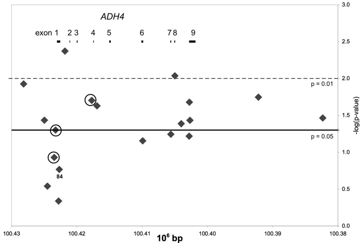
Figure 3. Association of SNPs across ADH4 with alcohol dependence defined by DSM-IV. Results of the PDT_{sum} are plotted as -\log(P\text{-value}) . The exons are indicated across the top. Nineteen SNPs in and immediately flanking ADH4 are shown (78–96 in Table 1; three SNPs further upstream were not significant). Circles mark the three SNPs that tag the associated haplotype, which runs from the second SNP through the last. SNP 84 is noted; this is the promoter SNP at -136 bp.
